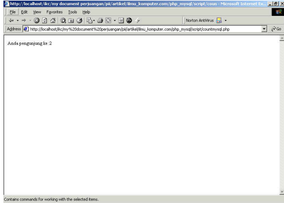
Gambar 22: Preview counter.php
