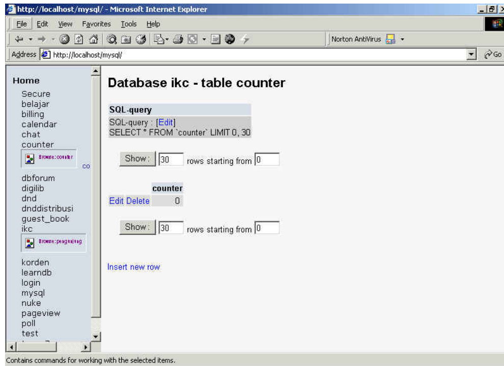
Gambar 21: Tabel counter
