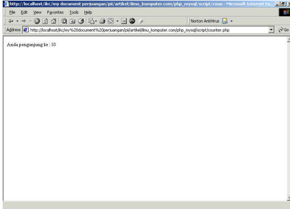
Gambar 20: Counter.php
