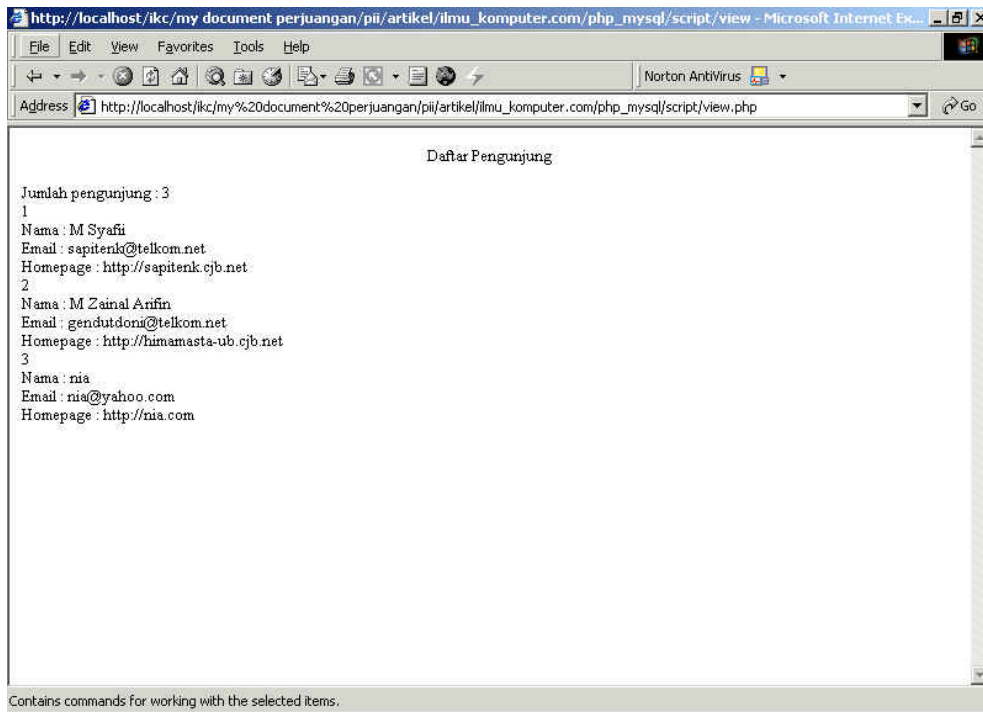
Gambar 13: Tambahan record
