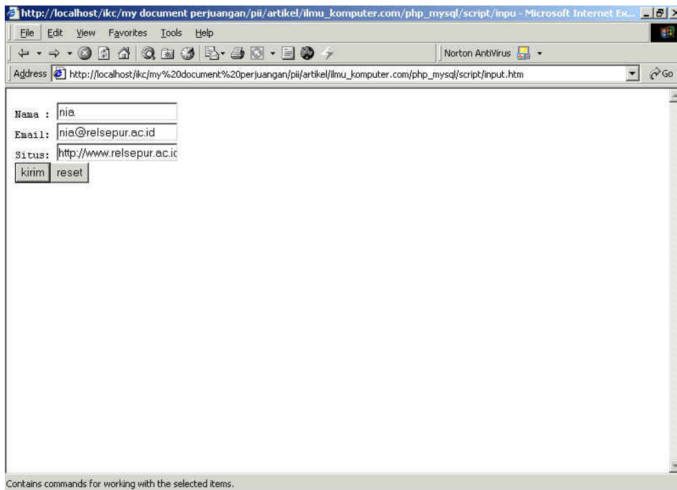
Gambar 11: Input data
