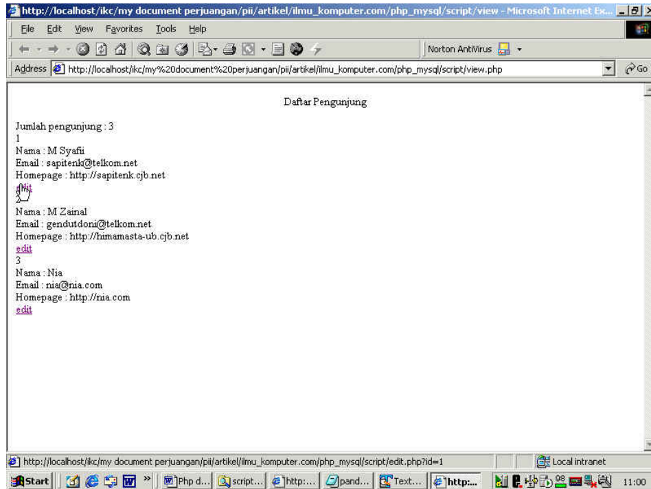
Gambar 14: View.php
