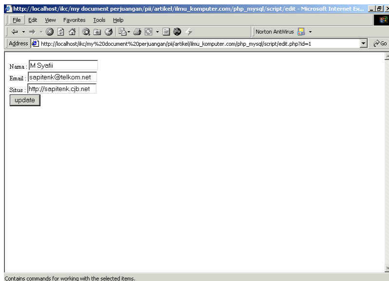
Gambar 15: edit.php?id=1
