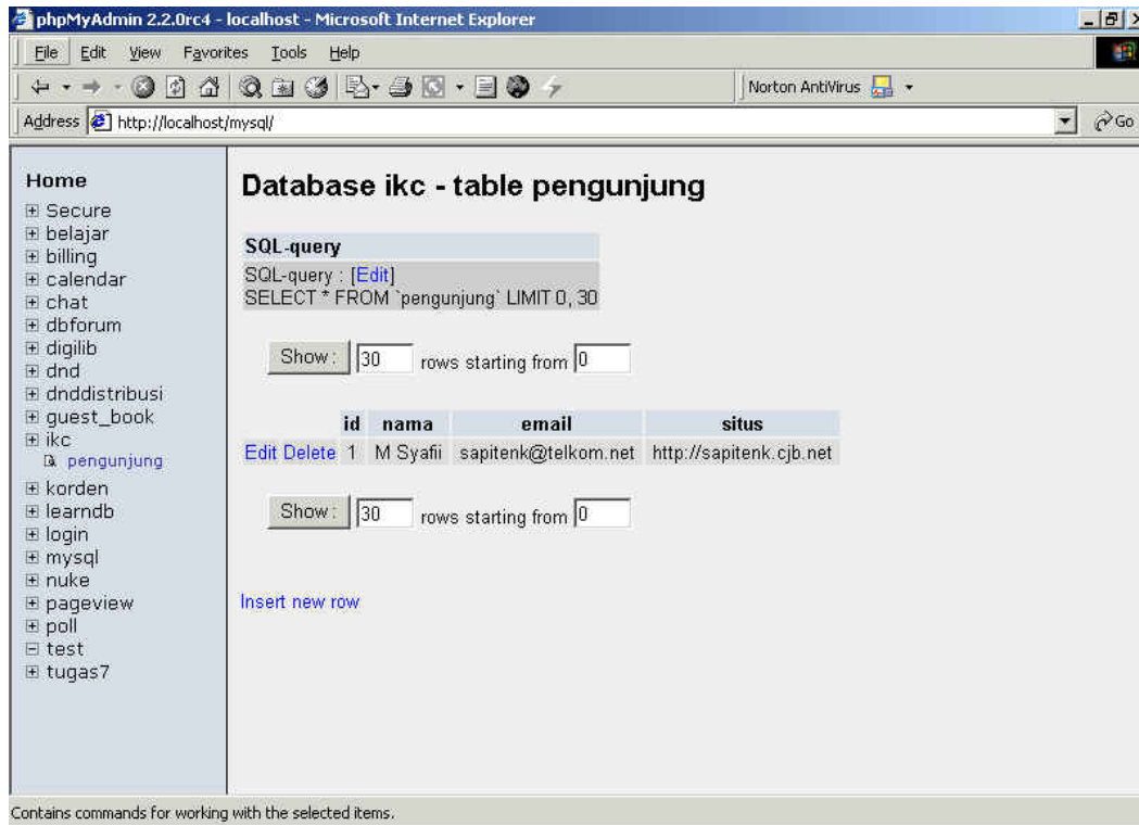
Gambar 7: Browse tabel
